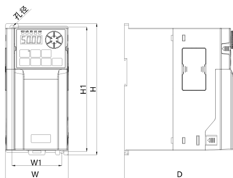
(a) S2 全部&T3-(0R4G-1R5G)
